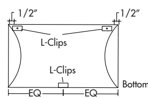
HORIZONTAL - REAR VIEW
