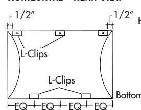
HORIZONTAL - REAR VIEW
