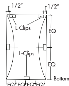
VERTICAL - REAR VIEW
