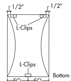
VERTICAL - REAR VIEW
