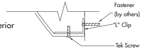
SIDE & BOTTOM "L" CLIP
