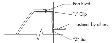
TOP "L" CLIP
