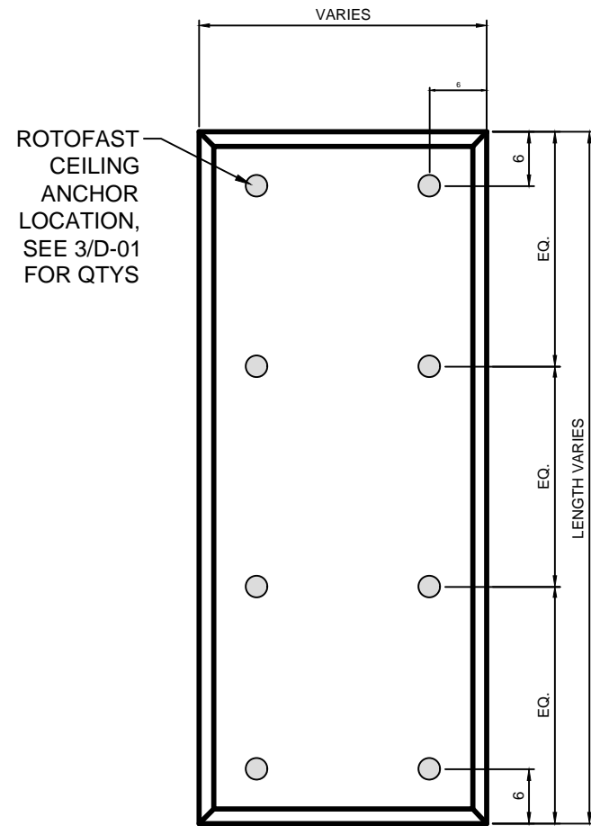
1 D-01 ROTOFAST CEILING ANCHOR ATTACHMENT SCALE: NA
