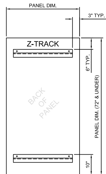
1 CX-05 Z-TRACK ATTACHMENT 72" & UNDER SCALE: NA
