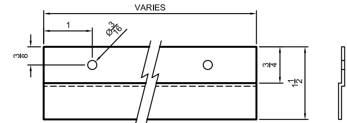
6 CX-05 Z-TRACK DETAIL SCALE: NA
