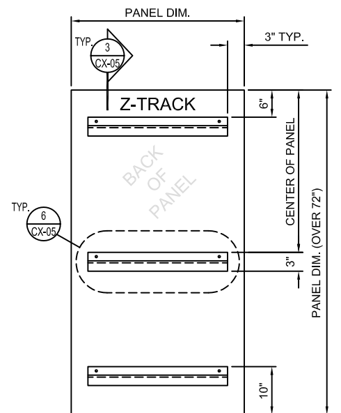
2 CX-05 Z-TRACK ATTACHMENT OVER 72" SCALE: NA
